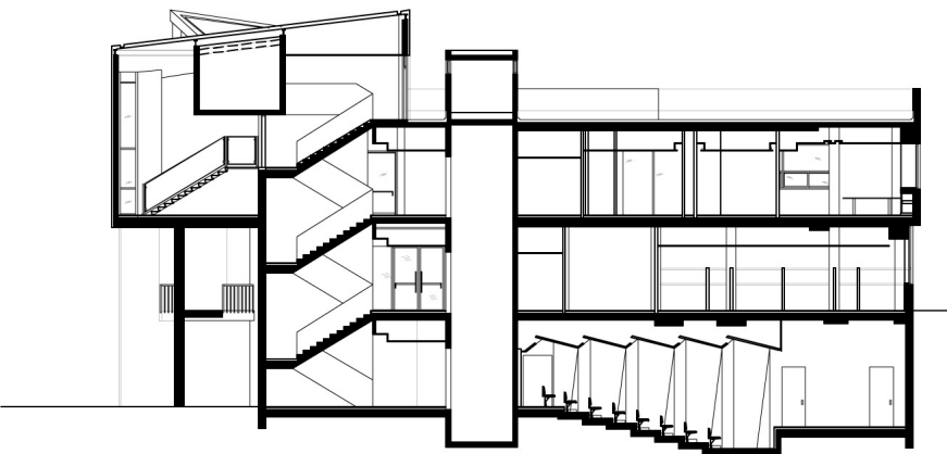
B-B SEC
