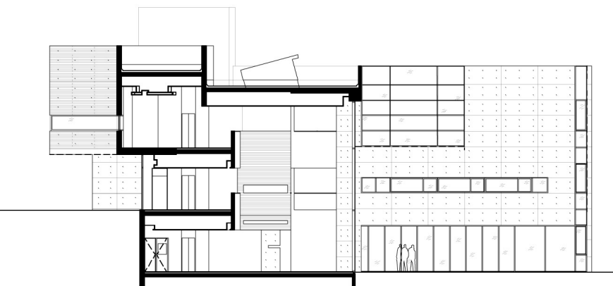
C-C SEC
